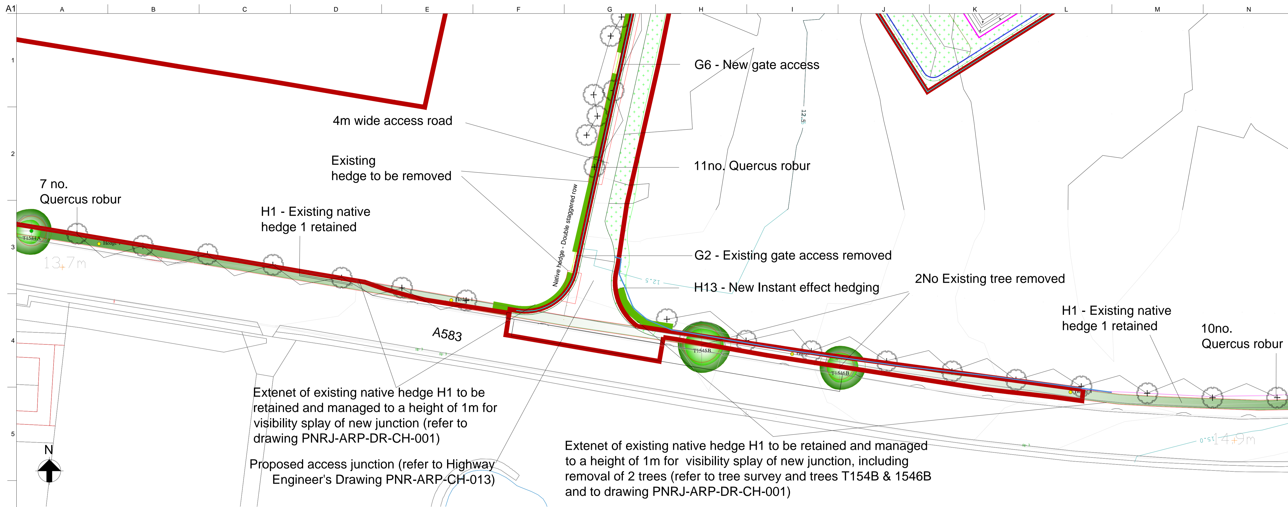
COMPOUND ENTRANCE JUNCTION WITH PRESTON NEW ROAD 1:500@A1
